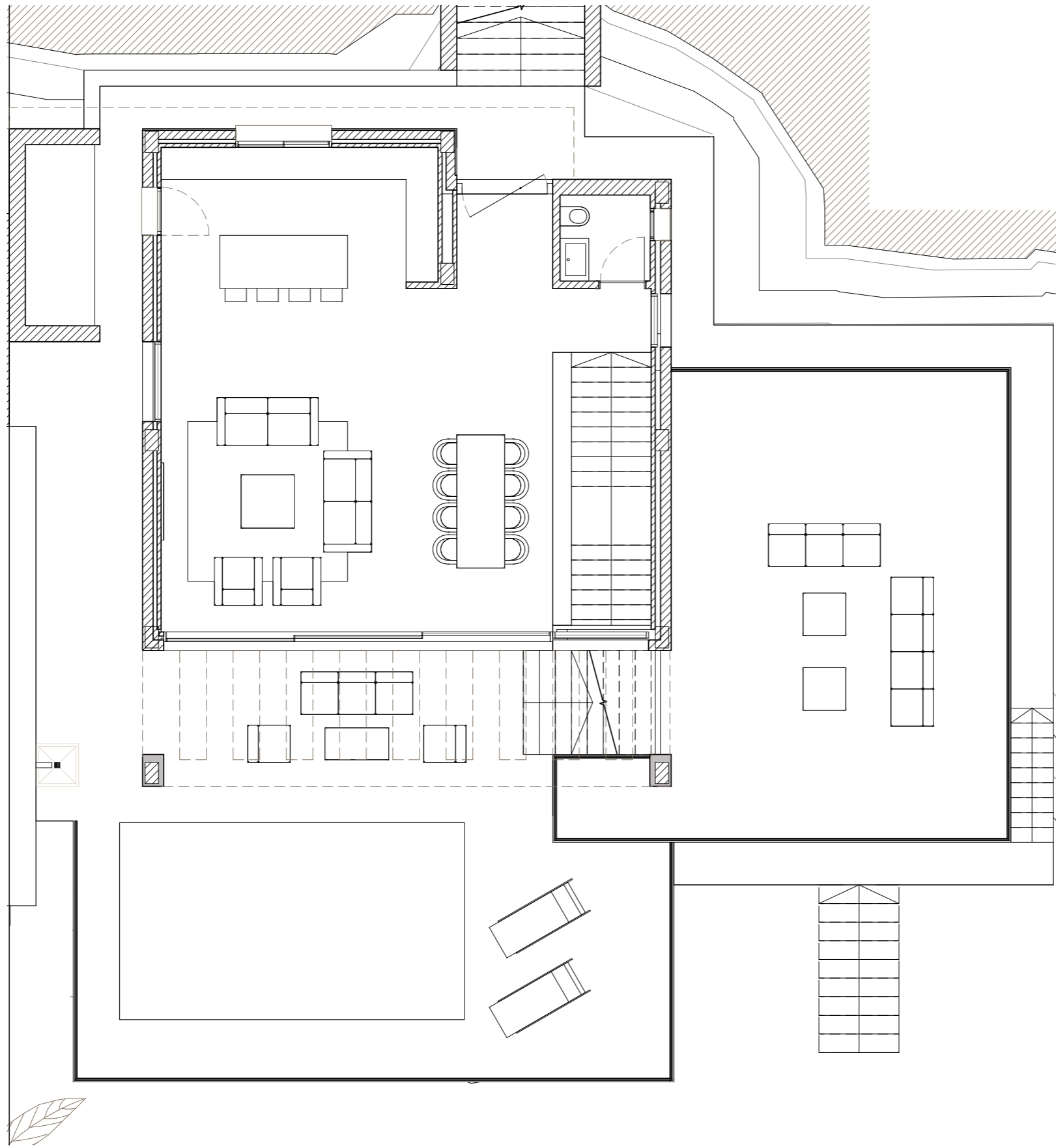
GROUND FLOOR
