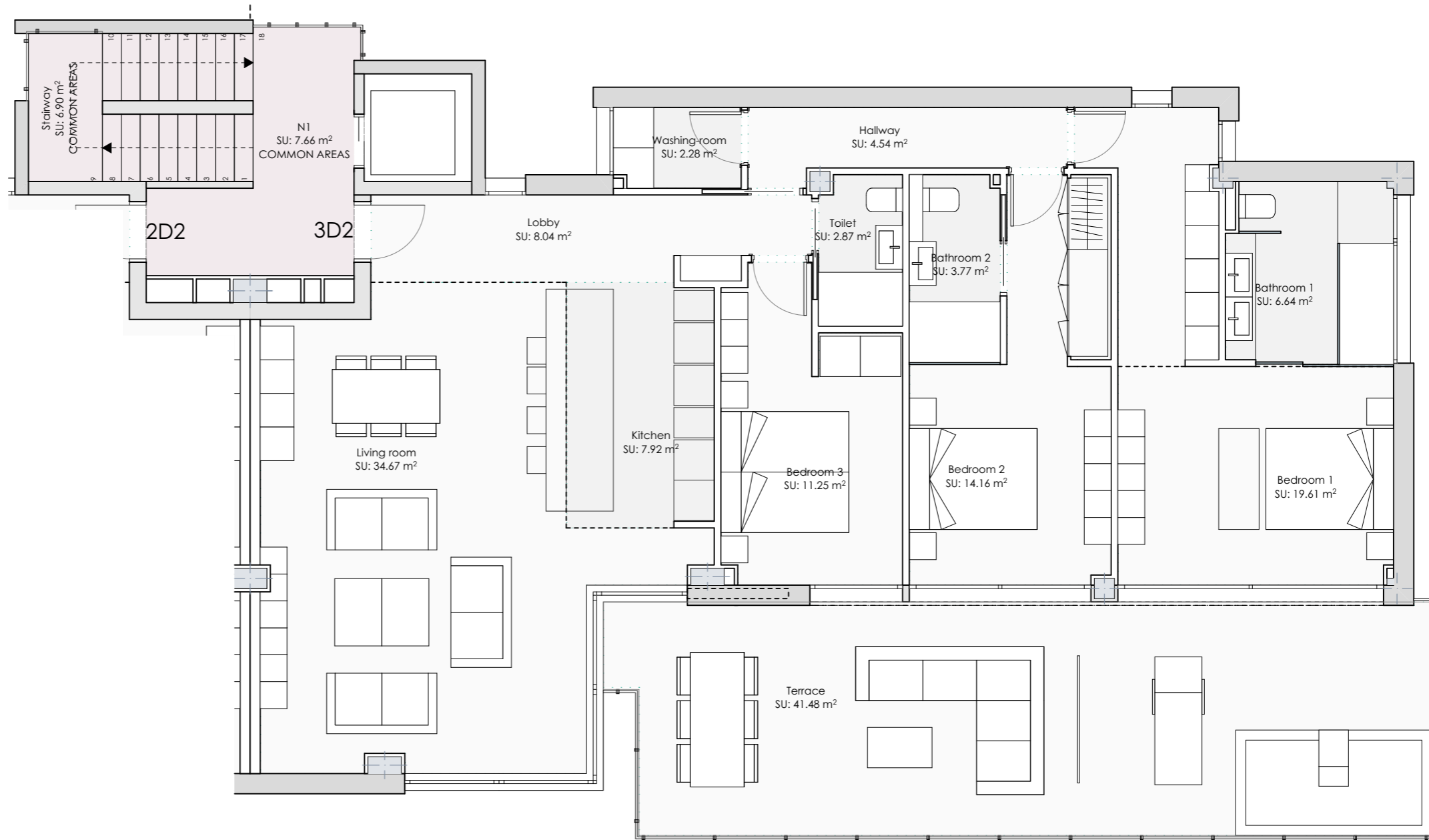
1- FIRST FLOOR
