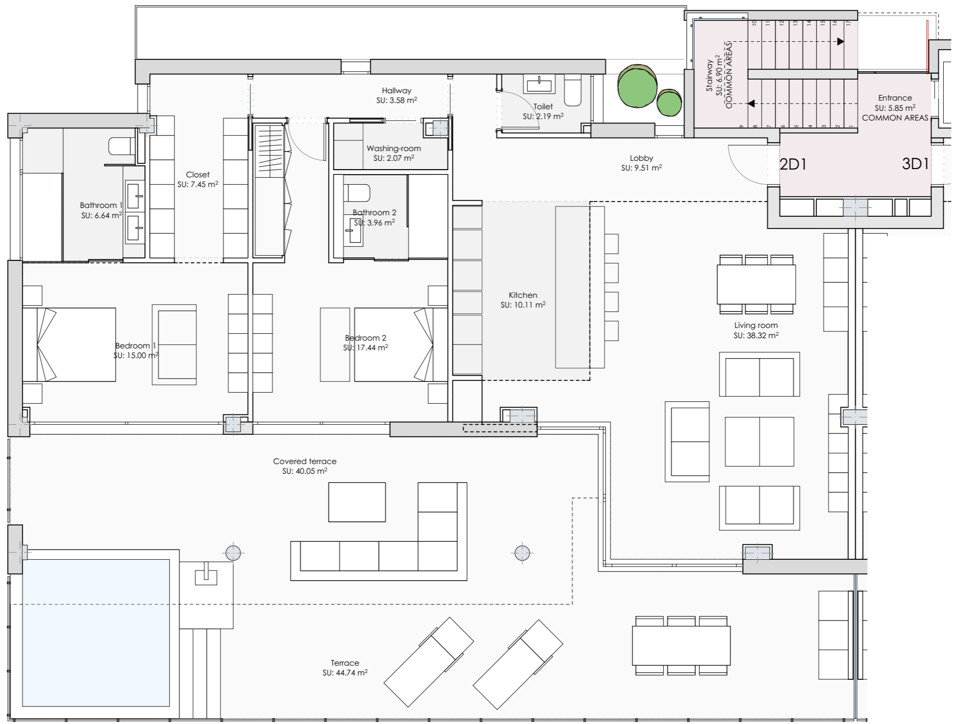
0- GROUND FLOOR
