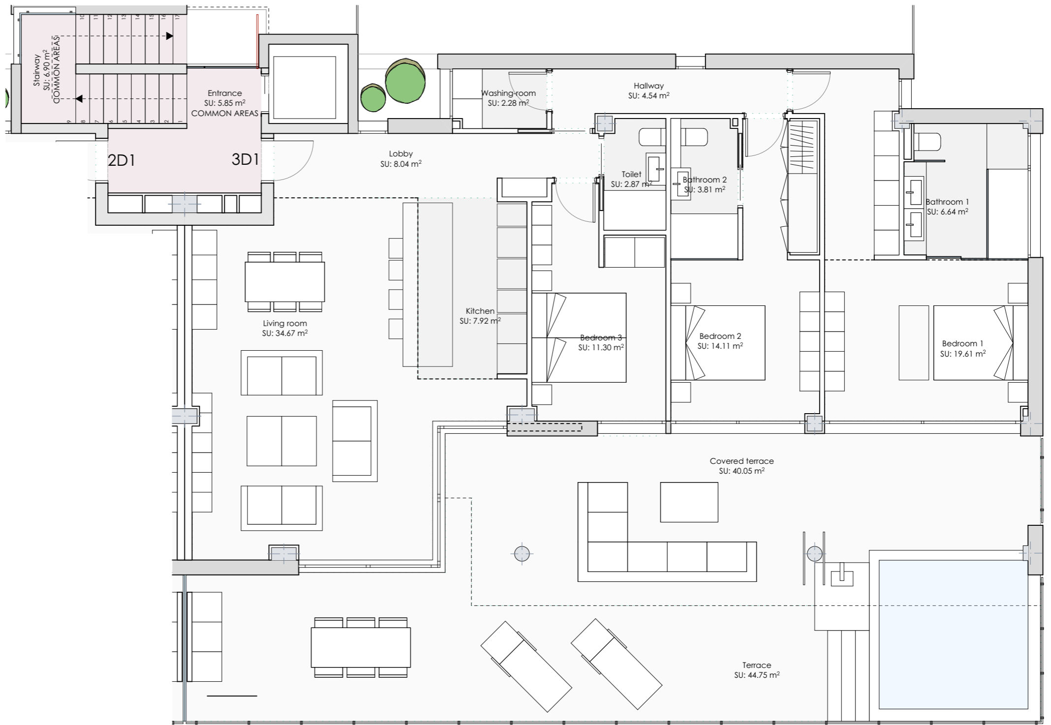
0- GROUND FLOOR
